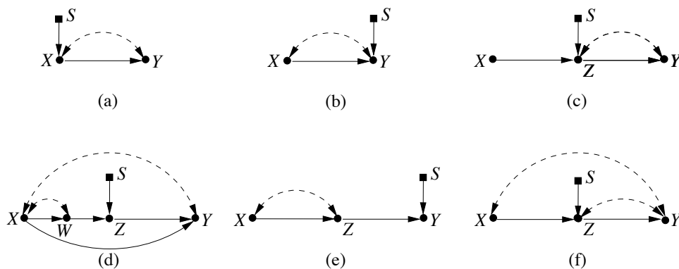
FIG 6. Selection diagrams illustrating transportability. The causal effect P(y|do(x)) is (trivially) transportable in (c) but not in (b) and (f). It is transportable in (a), (d), and (e) (see Corollary 2).
