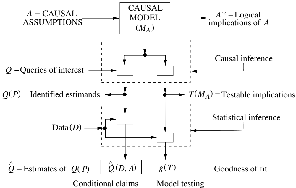
Figure 1: SEM methodology depicted as the an inference engine converting assumptions ( A ), queries ( Q ), and data ( D ) into logical implications ( A^* ), conditional claims ( C ), and data-fitness indices ( g(T) ).
