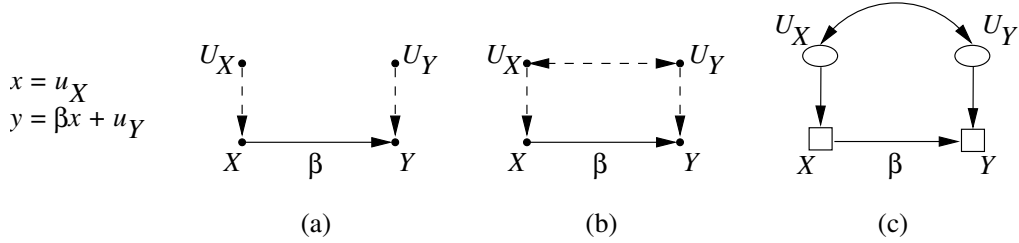
Figure 2: A simple structural equation model, and its associated diagrams, showing (a) independent unobserved exogenous variables (connected by dashed arrows), (b) dependent unobserved exogenous variables, and (c) an equivalent, more traditional notation, in which latent variables are enclosed in ovals.
