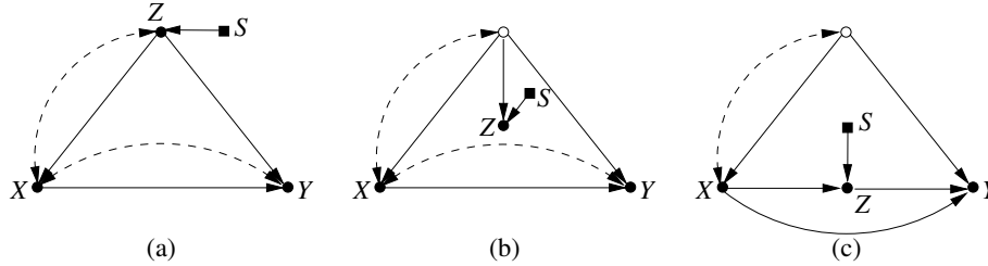
Figure 9: Selection diagrams depicting differences in populations. In (a), the two populations differ in age distributions. In (b), the populations differs in how reading skills ( Z ) depends on age (an unmeasured variable, represented by the hollow circle) and the age distributions are the same. In (c), the populations differ in how Z depends on X .
